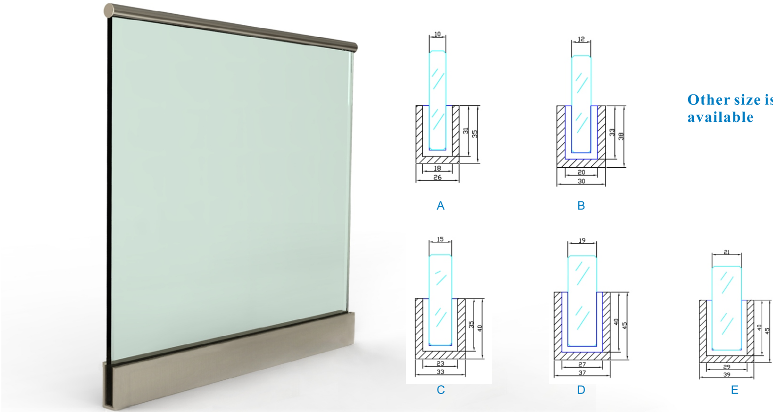
Round Channel Pipe And Base Profile System
