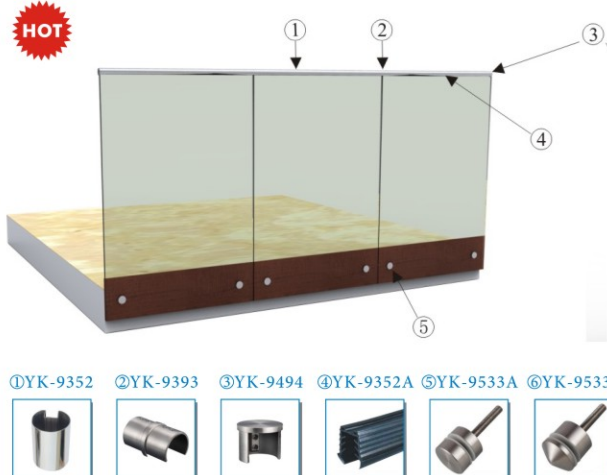
Model: Semi Glass Fense Spigot System(Round/Square Spigots)
